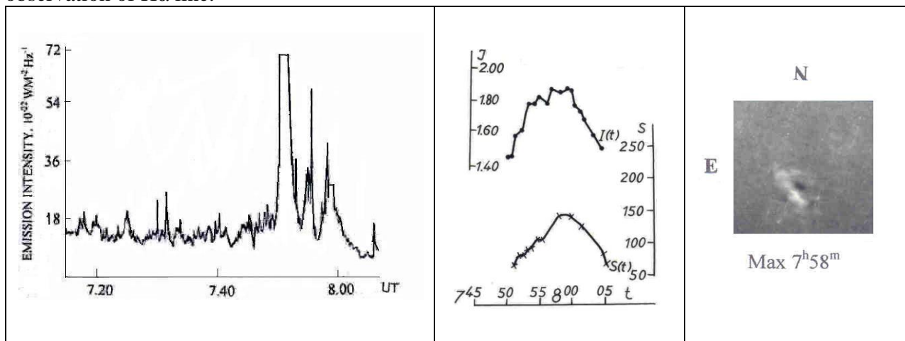
Figure 7. Observations of a flare № 7. In the figure on the left, we can see a change in the radio flow. The diagram in the center shows the intensity and area of the flare. The photo on the right is the observation of H \alpha line.
