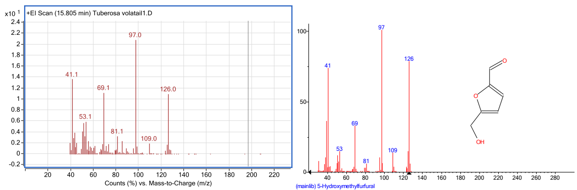
სურ. №4. 15,8 - 5-Hydroxymethylfurfural
