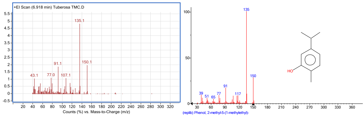
სურ. №17. 6,91 – Carvacrol: 2 – methyl – 5 (1-methylethyl) phenol
