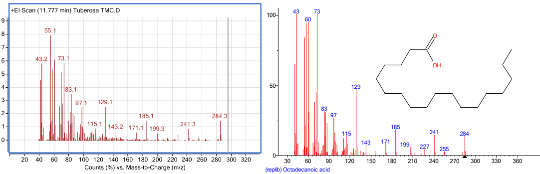
სურ. №11. 11,77 - Stearic acid, Octadecanoic acid
