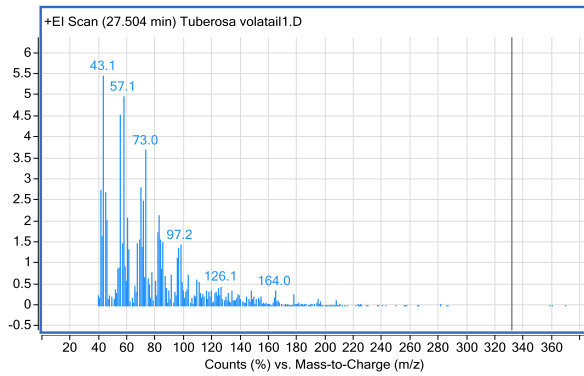
სურ. 11. 27,5 - 3-hydroxy Dodecanoic acid
