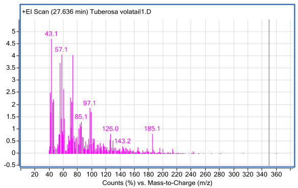
სურ.№12. 27,63 - D-Melezitose: α-D-Glucopyranoside, O-α-D – Glucopyranosyle-β – D-fructofuranosyle
