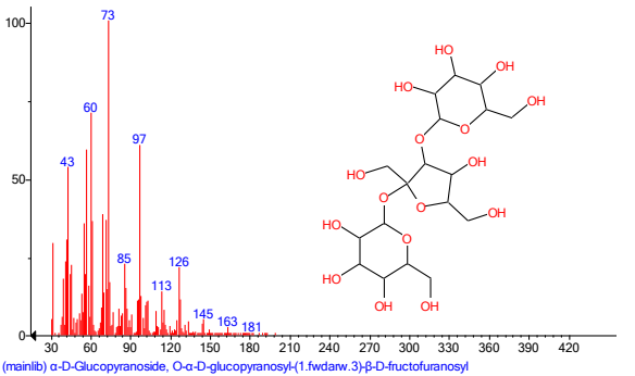
სურ.№12. 27,63 - D-Melezitose: α-D-Glucopyranoside, O-α-D – Glucopyranosyle-β – D-fructofuranosyle
