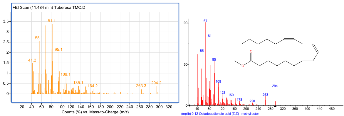
სურ. №19. 11,48 - Methyl linoleate: 9.12-octadecadienoic acid
