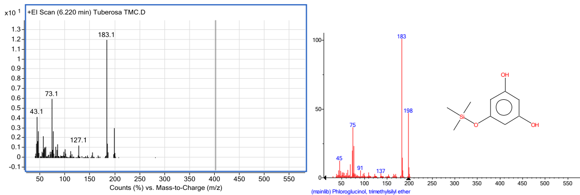
სურ. №15. 6,2 - Phloroglucinol: 1,3,5-trihydroxybenzol, Trimethylsilyl ether
