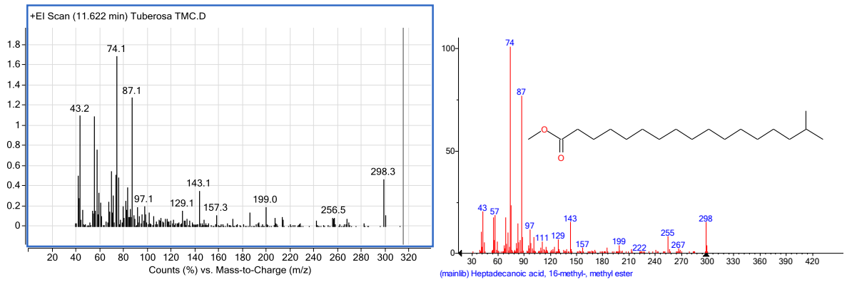
სურ. №20. 11,62 - Methyl isostearate: Heptadecanoic acid, 16-methyl-, methyl ester
