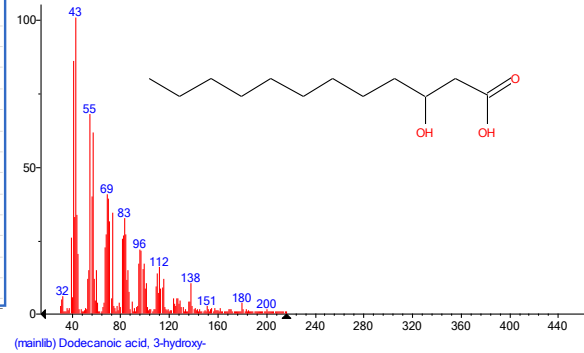
სურ. 11. 27,5 - 3-hydroxy Dodecanoic acid
