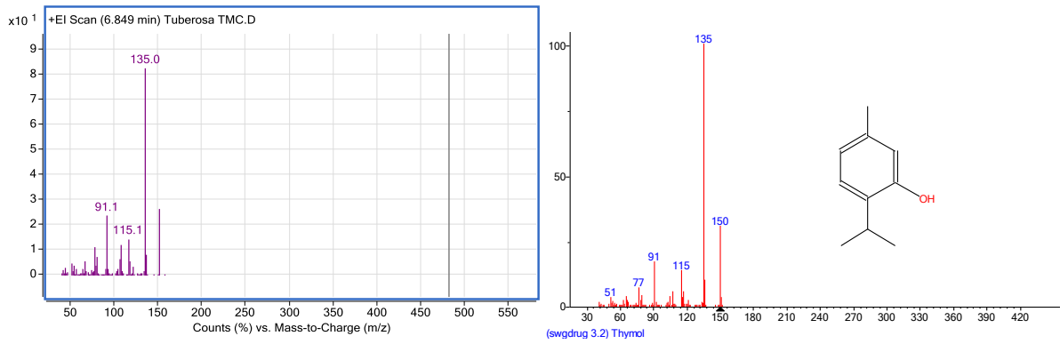
სურ. №16. 6,85 - Thymol: 2-isopropyl-5- methylphenol T
