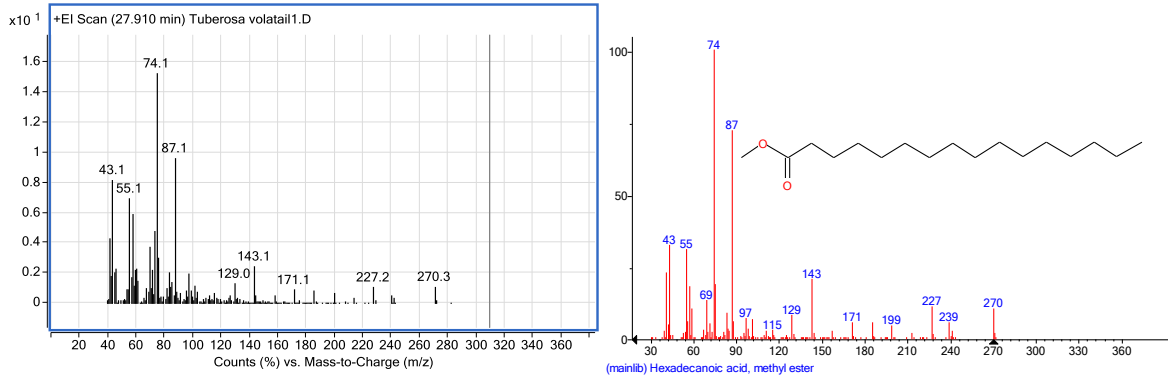
სურ. №13. 27,91 - Methyl palmitate: Methyl ester hexadecanoic acid
