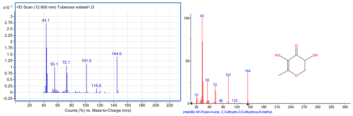
სურ. №2. 12,6 - Pyranone: 2,3-dihydro-3,5-dihydroxy-6-methyl-4(H)-Pyran-4-one
