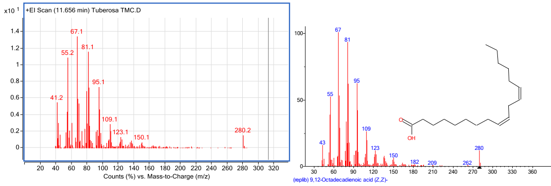
სურ. №21. 11,65 - Linoleic acid: 9,12 - Octadecadienoic acid
