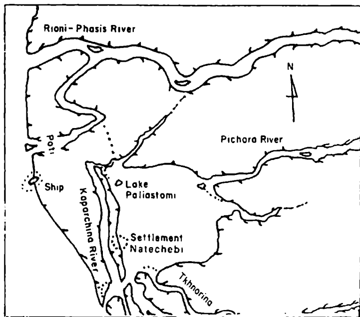
Figure 2 Map of Phasis (Poti) and the Lake Paliastomi area
